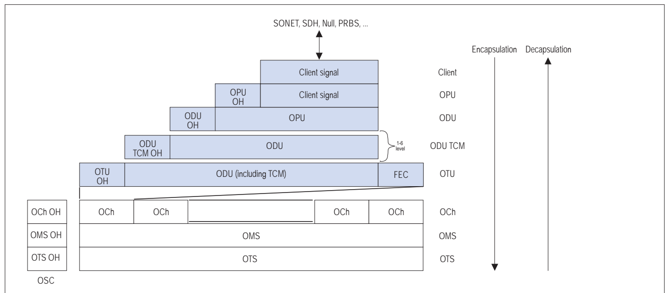
Figure 2: Basic OTN Transport Structure
