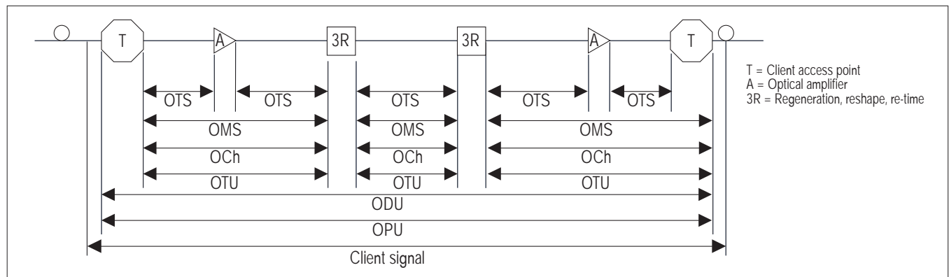
Figure 1: OTN Layer Termination Points
