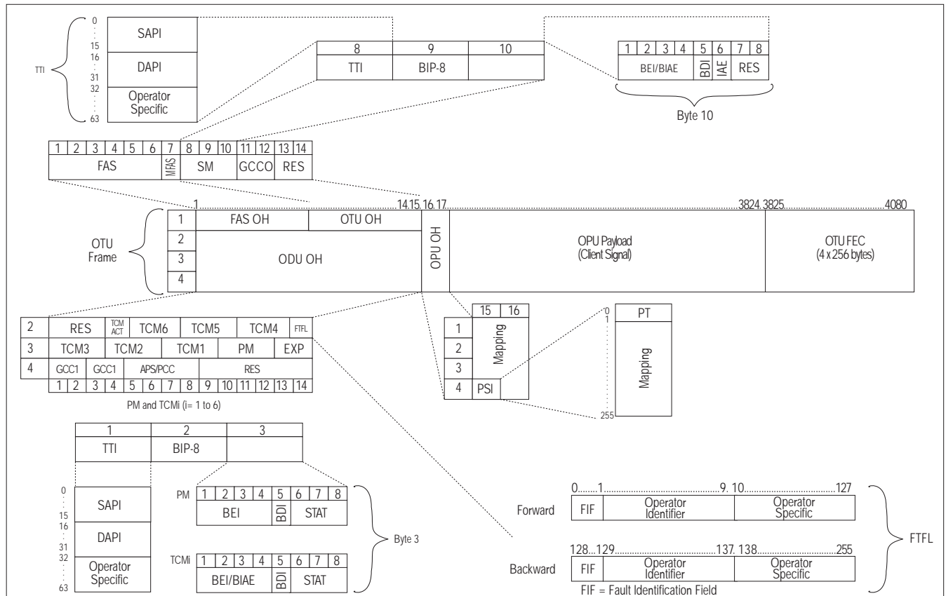
Figure 3: OTU Frame Description
