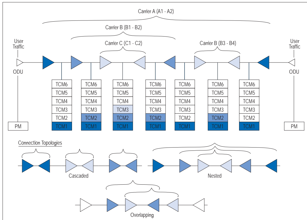
Figure 4: Tandem Connection Monitoring
