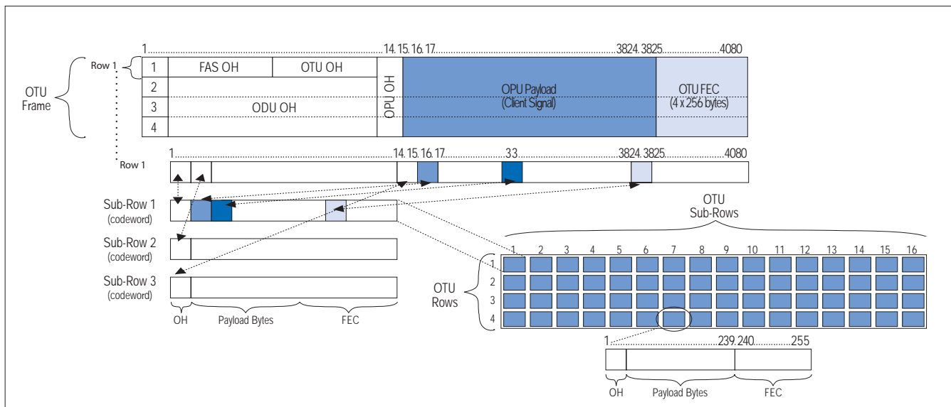
Figure 5: Forward Error Correction
