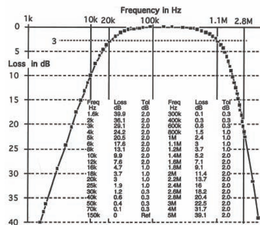
Figure 1 - G Filter for the ADSL
